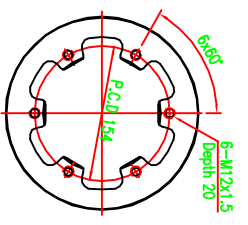
Detail of Crank Shaft Pulley
