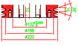
Detail of Crank Shaft Pulley
